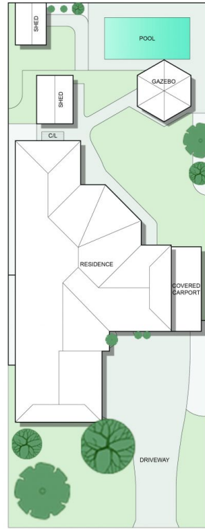
HORIZON DRIVE SITE PLAN
