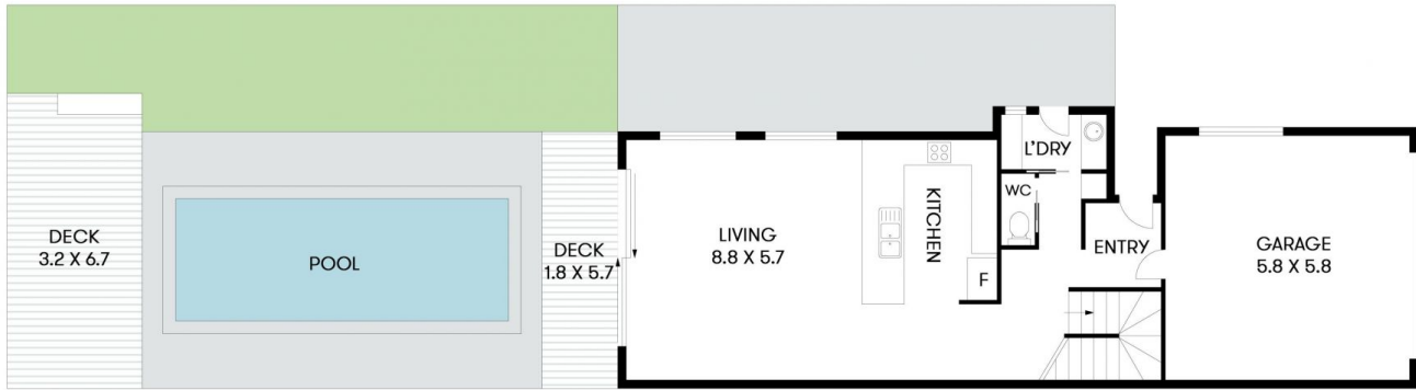
GROUND FLOOR
