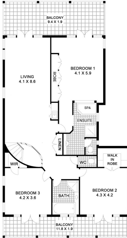
UPPER FLOOR
